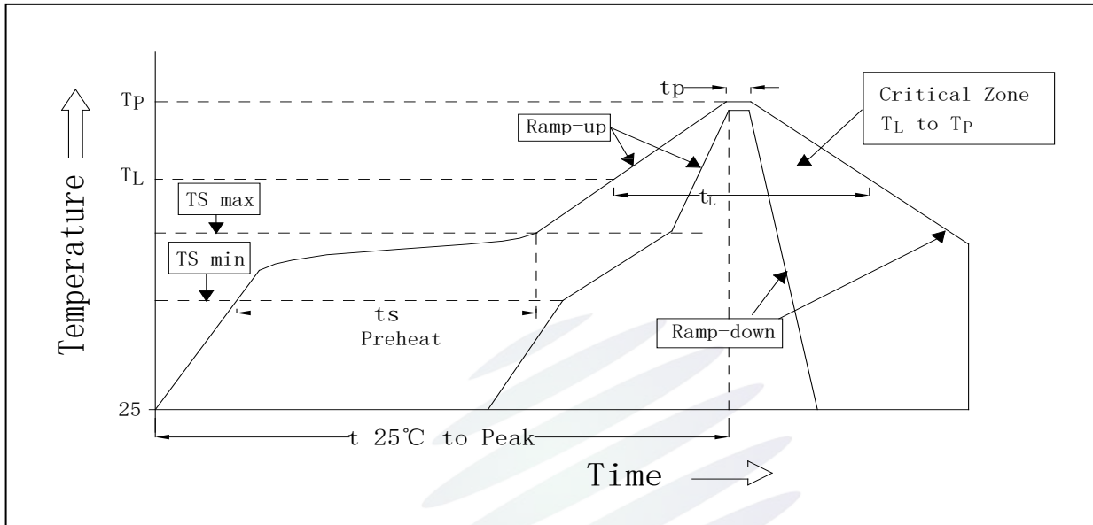
Fig.3-1 SMT Reflow Soldering Instructions SMT 回流焊说明
