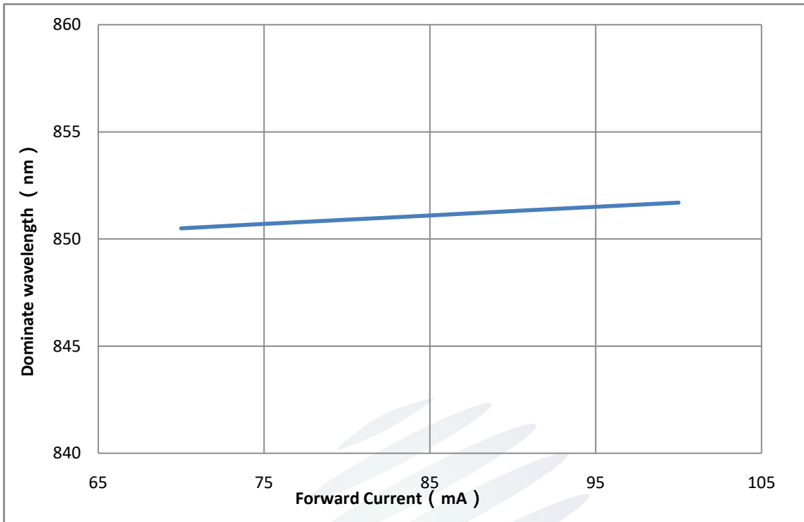
Fig. 1-13 Forward current vs.Dominate wavelength (Ts=25°C)正向电流与主导波长特性曲线(Ts=25°C)
