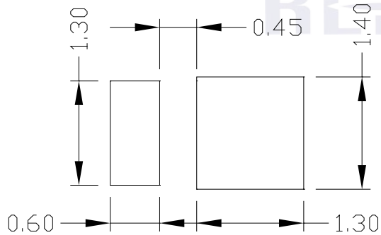
Fig.1-5 Soldering Patterns 推荐焊盘
