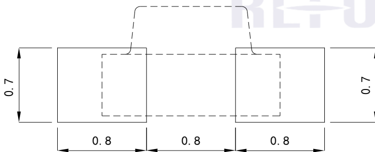
Fig.1-5 Soldering patterns 推荐焊盘
