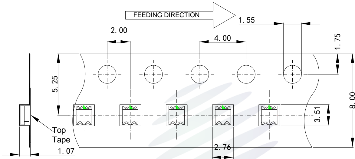
Fig.2-1 Carrier Tape Dimension 载带尺寸
